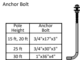
Anchor Bolt
