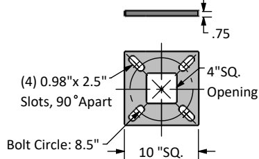
LED Fixture Front View
