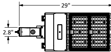
LED Fixture
