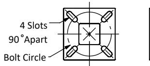
Base Plate
