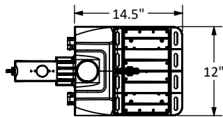
LED Fixture Top view
