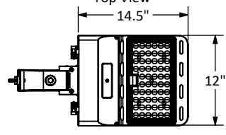
LED Fixture Bottom View
