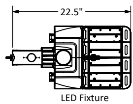
LED Fixture Top View
